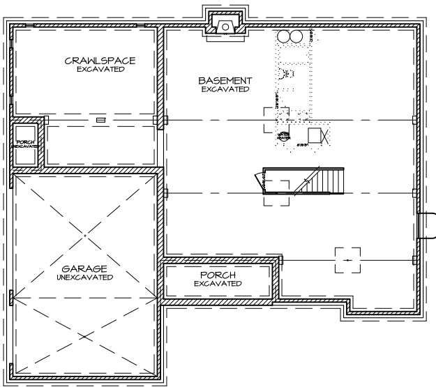
FOUNDATION PLAN A-4
