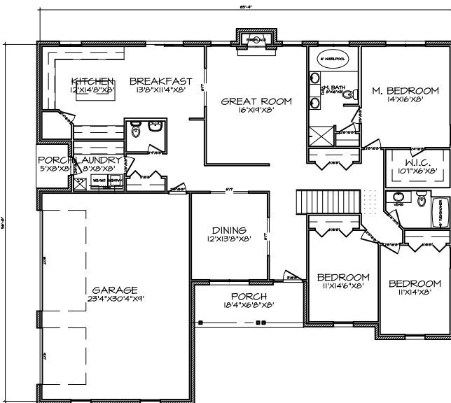
FIRST FLOOR PLAN A-2
